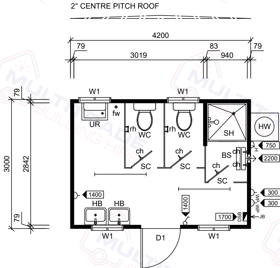
4.2x3.0m Ablution - Floor Plan
